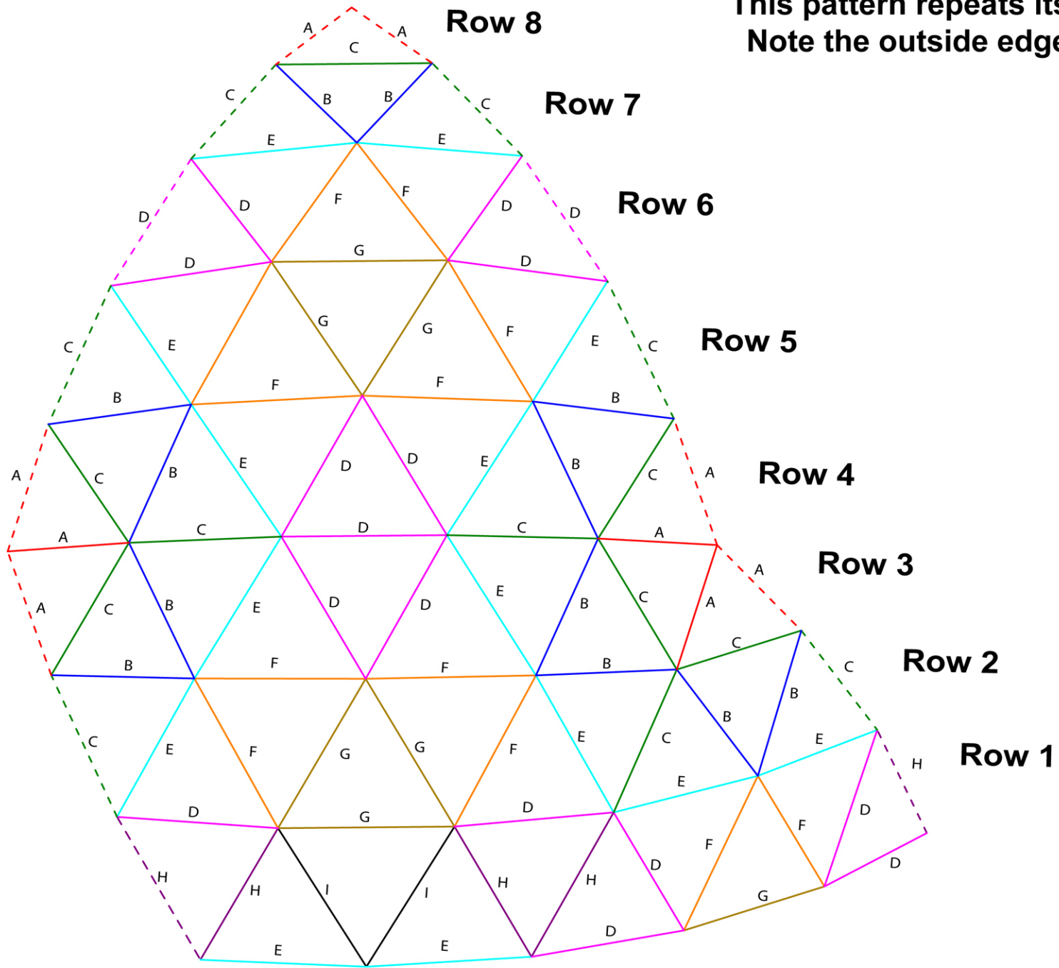
36' DOME FRAME DIAGRAM
