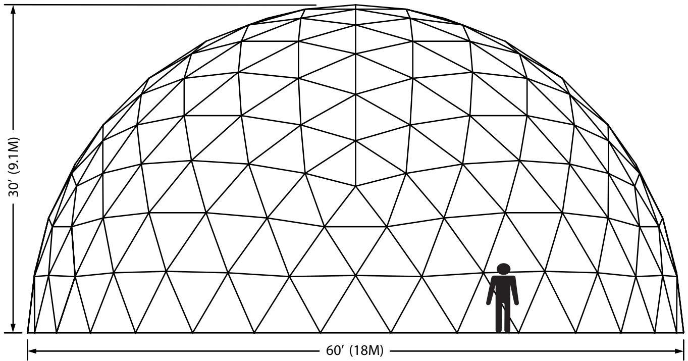
60' Dome Elevation
