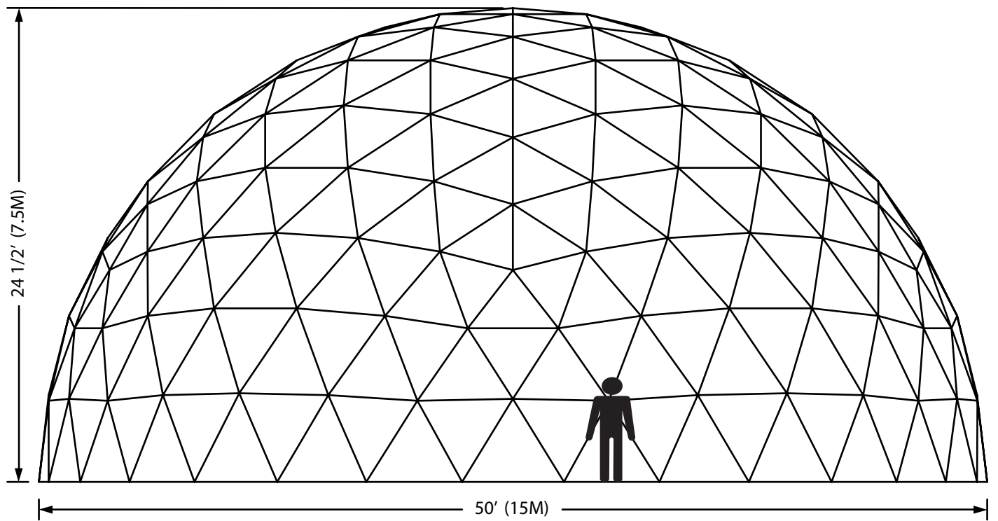
50' Dome Elevation
