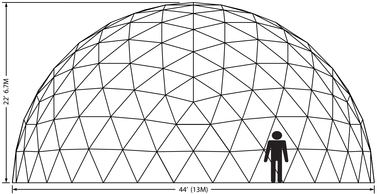
44' Dome Elevation
