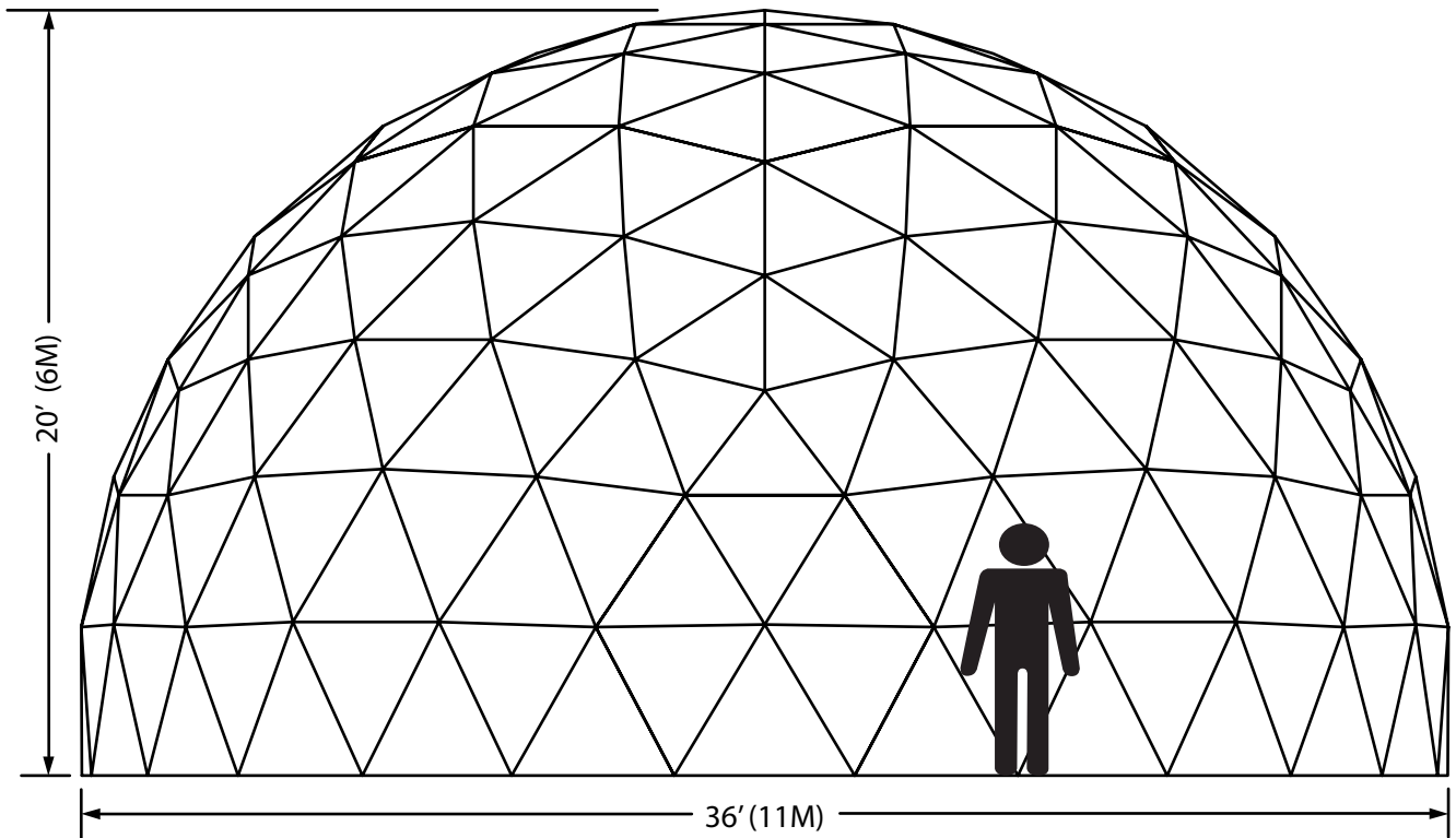
36' Dome Elevation
