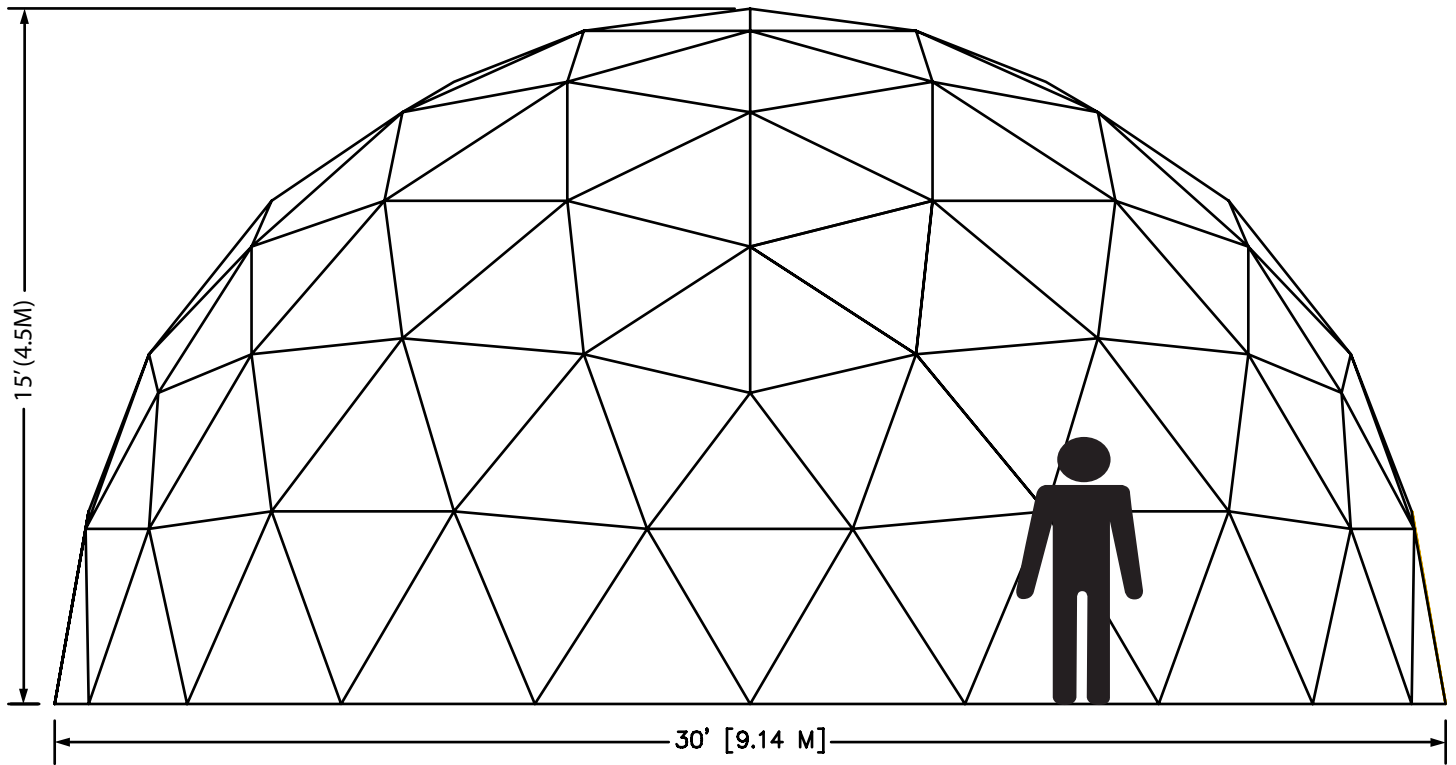
30' Dome Elevation
