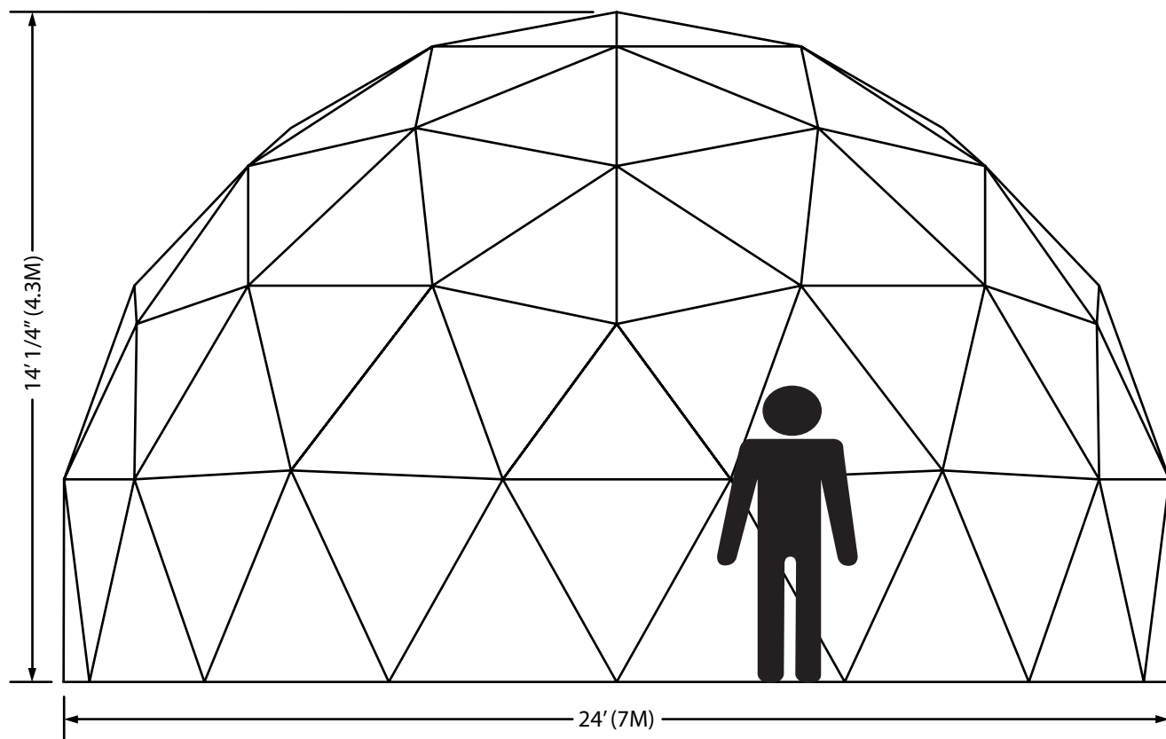
24' Dome Elevation
