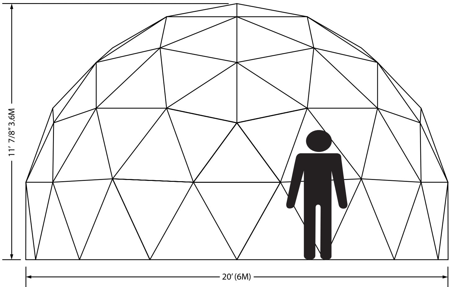
20' Dome Elevation
