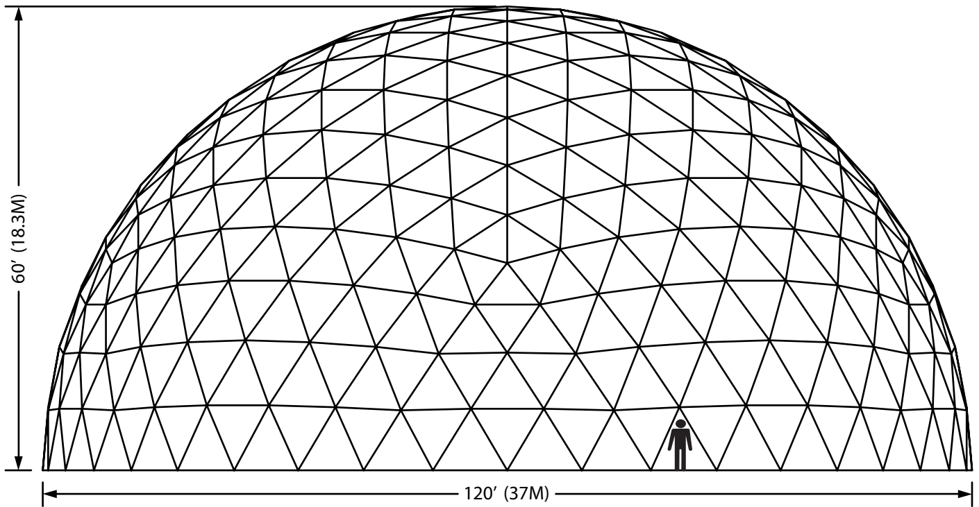
120' Dome Elevation
