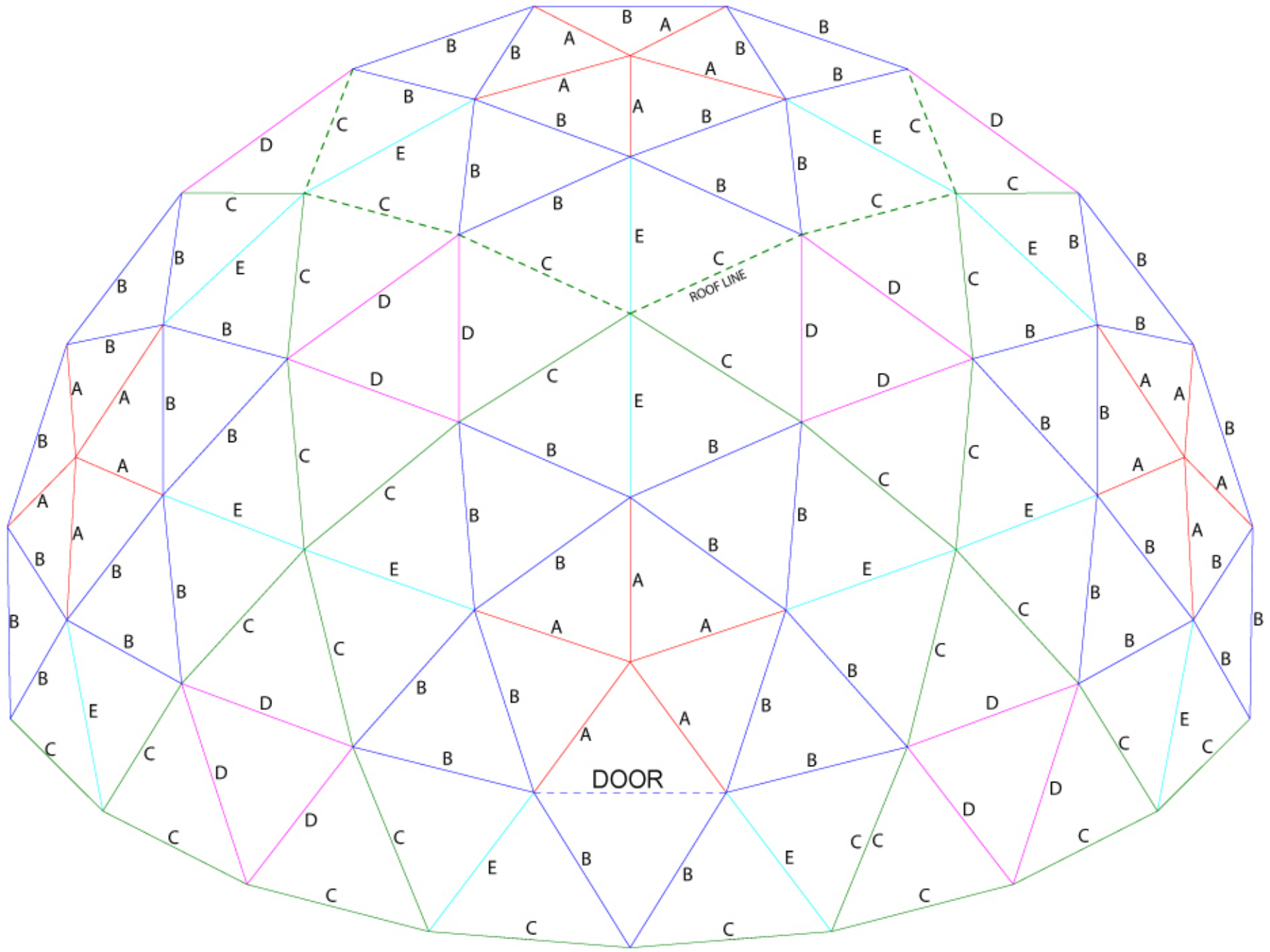
30' DOME - STRUT LOCATIONS
